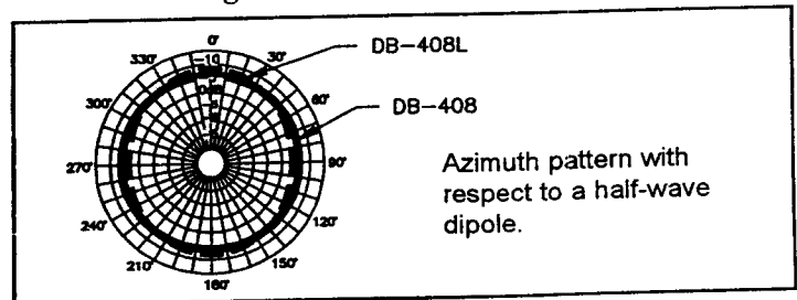
Figure 4 - Azimuth Pattern
